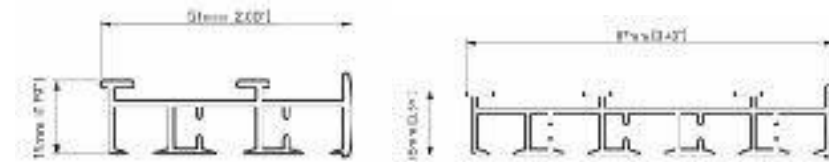
4 CHANNEL
